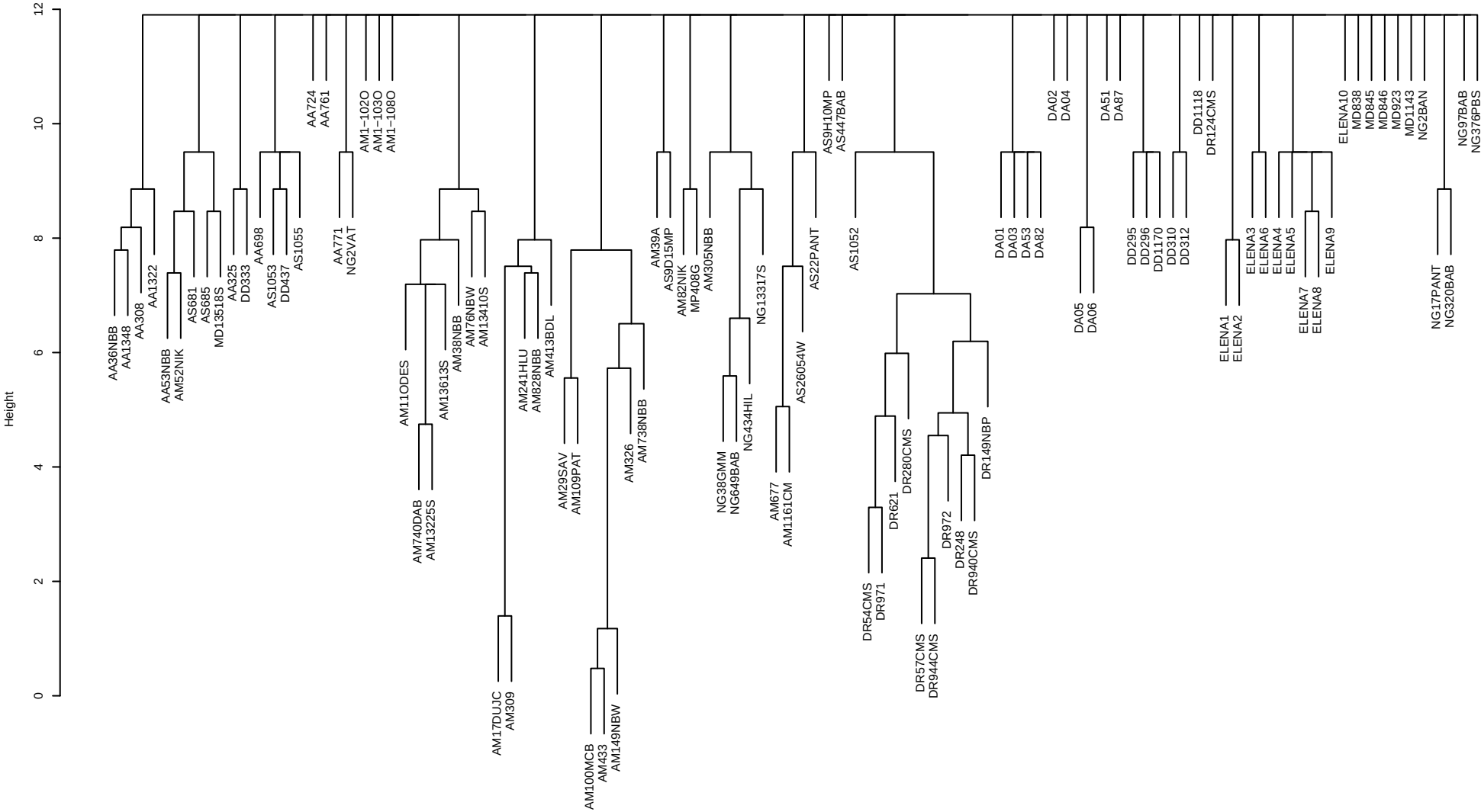
Dendrogram of agnes(x = logdis, diss = TRUE, method = "complete")
