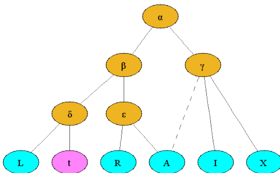
Figure 34: Example stemma
